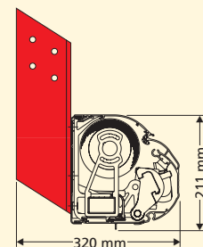
Rafter mounting
