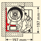
Niche installation
