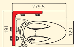
Ceiling mounting
