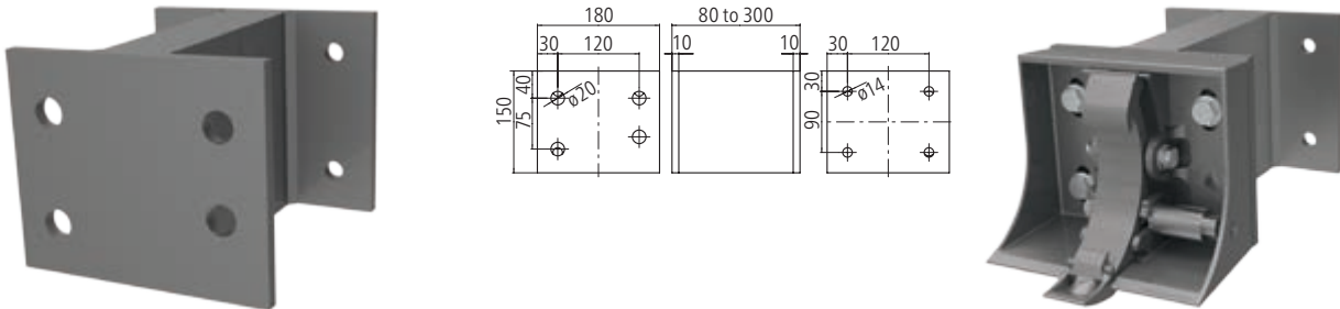
Stand off bracket
