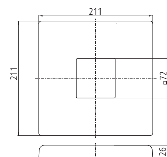
Post plate cover cap 211 x 211 x 26 mm
