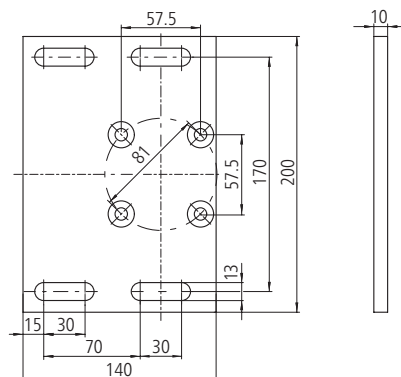
Post plate 200 x 140 x 10 mm
