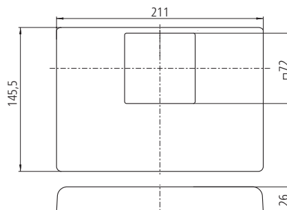
Post plate cover cap 211 x 145 x 26 mm
