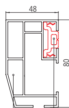
Fabric guide profile Side channel
