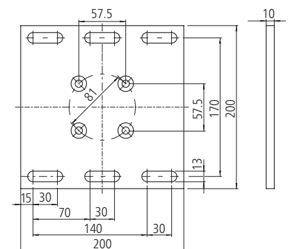
Post plate 200 x 200 x 10 mm
